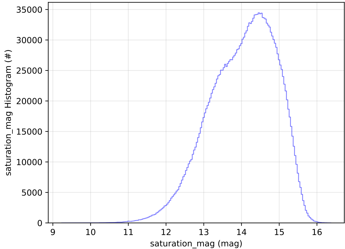
ddf_acor_sf10_lsf30_lsr10_v3.4_10yrs WFD all bands: saturation_mag Histogram
