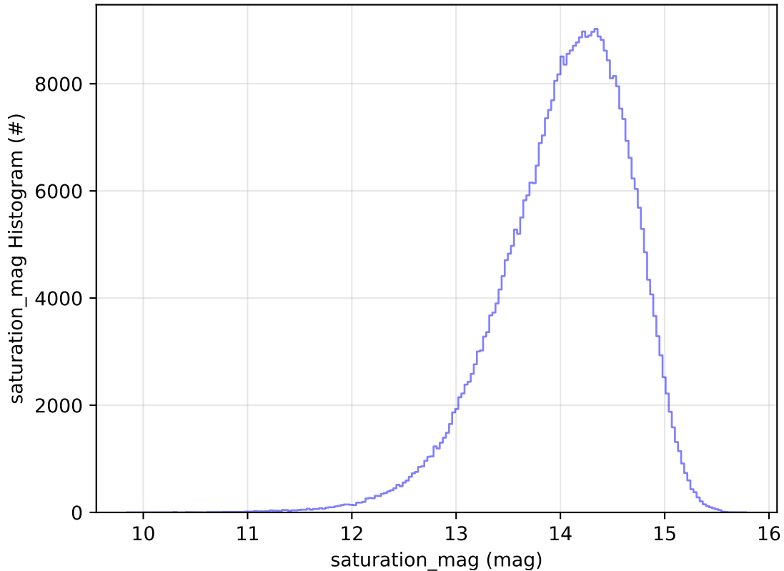
ddf_acor_sf10_lsf30_lsr10_v3.4_10yrs All sky z band: saturation_mag Histogram
