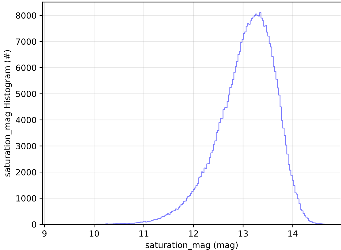
ddf_acor_sf10_lsf30_lsr10_v3.4_10yrs All sky y band: saturation_mag Histogram
