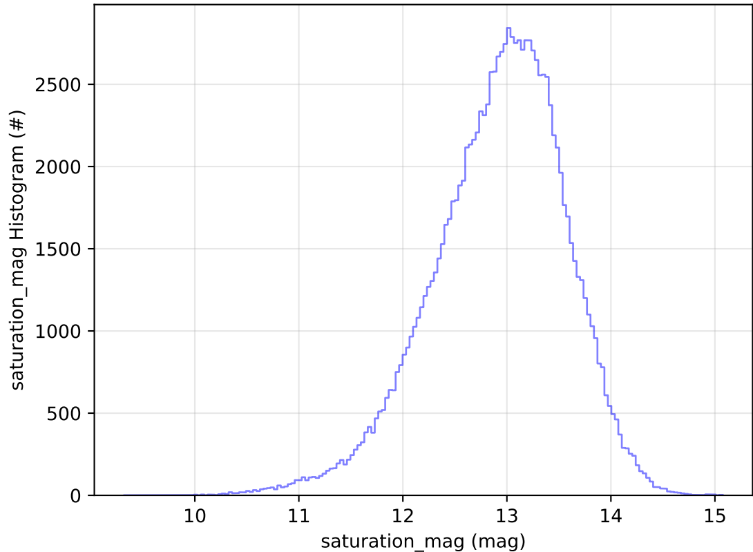
ddf_acor_sf10_lsf30_lsr10_v3.4_10yrs All sky u band: saturation_mag Histogram
