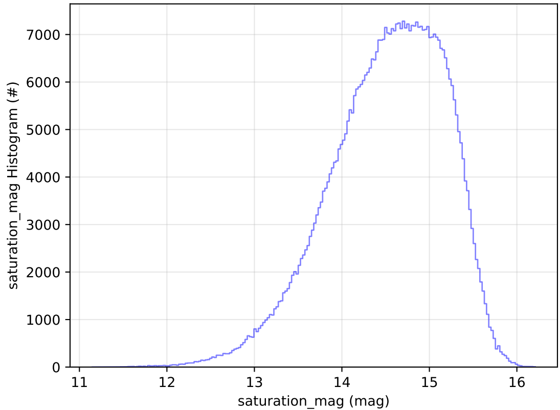
ddf_acor_sf10_lsf30_lsr10_v3.4_10yrs All sky r band: saturation_mag Histogram
