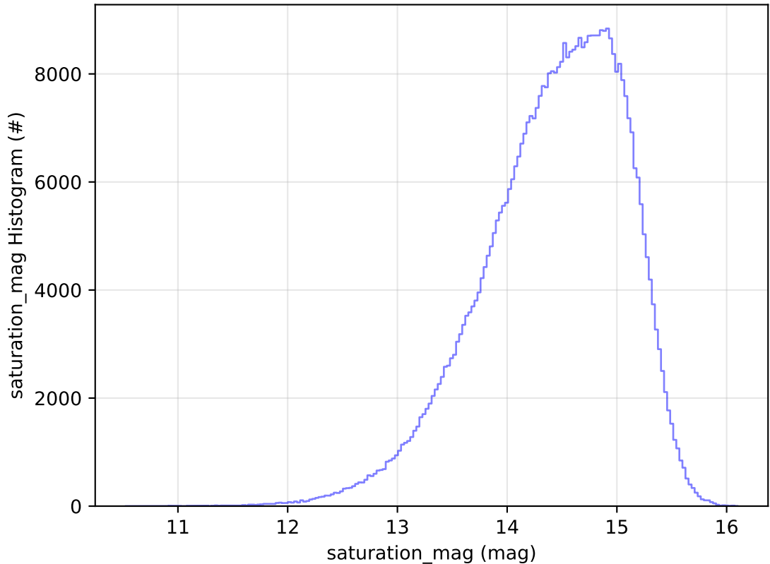
ddf_acor_sf10_lsf30_lsr10_v3.4_10yrs All sky i band: saturation_mag Histogram
