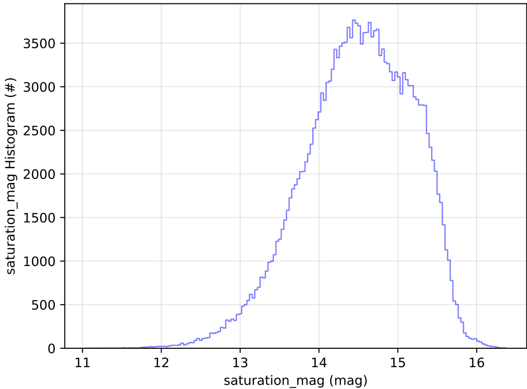
ddf_acor_sf10_lsf30_lsr10_v3.4_10yrs All sky g band: saturation_mag Histogram
