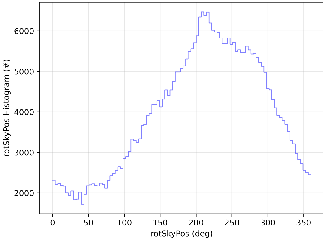
ddf_acor_sf10_lsf30_lsr10_v3.4_10yrs WFD y band: rotSkyPos Histogram
