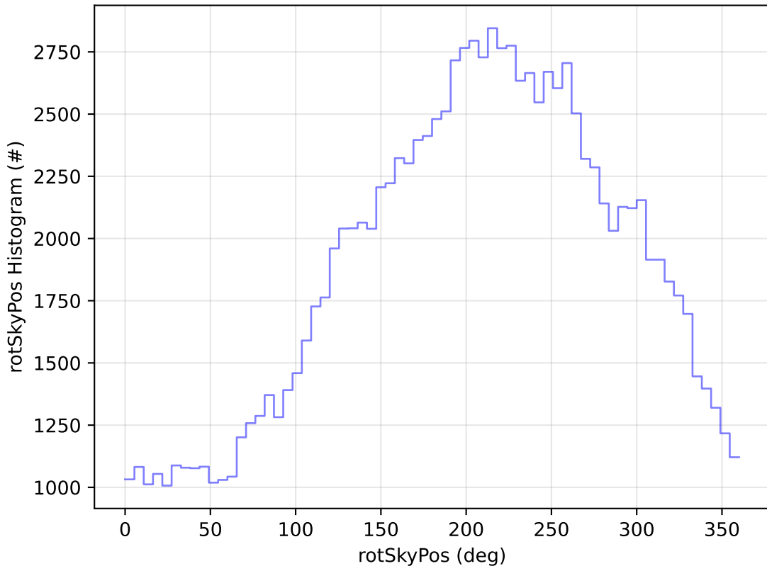
ddf_acor_sf10_lsf30_lsr10_v3.4_10yrs WFD u band: rotSkyPos Histogram
