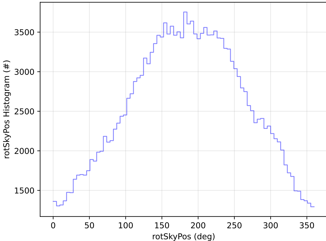
ddf_acor_sf10_lsf30_lsr10_v3.4_10yrs WFD g band: rotSkyPos Histogram
