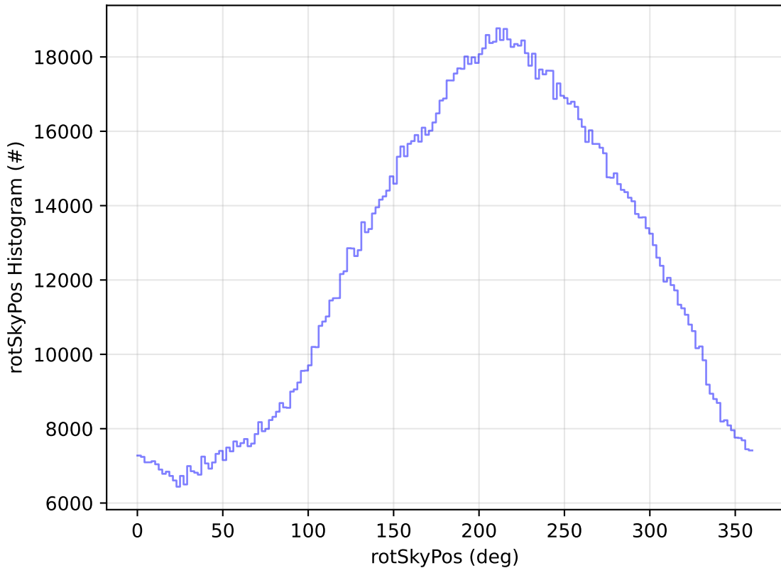
ddf_acor_sf10_lsf30_lsr10_v3.4_10yrs WFD all bands: rotSkyPos Histogram
