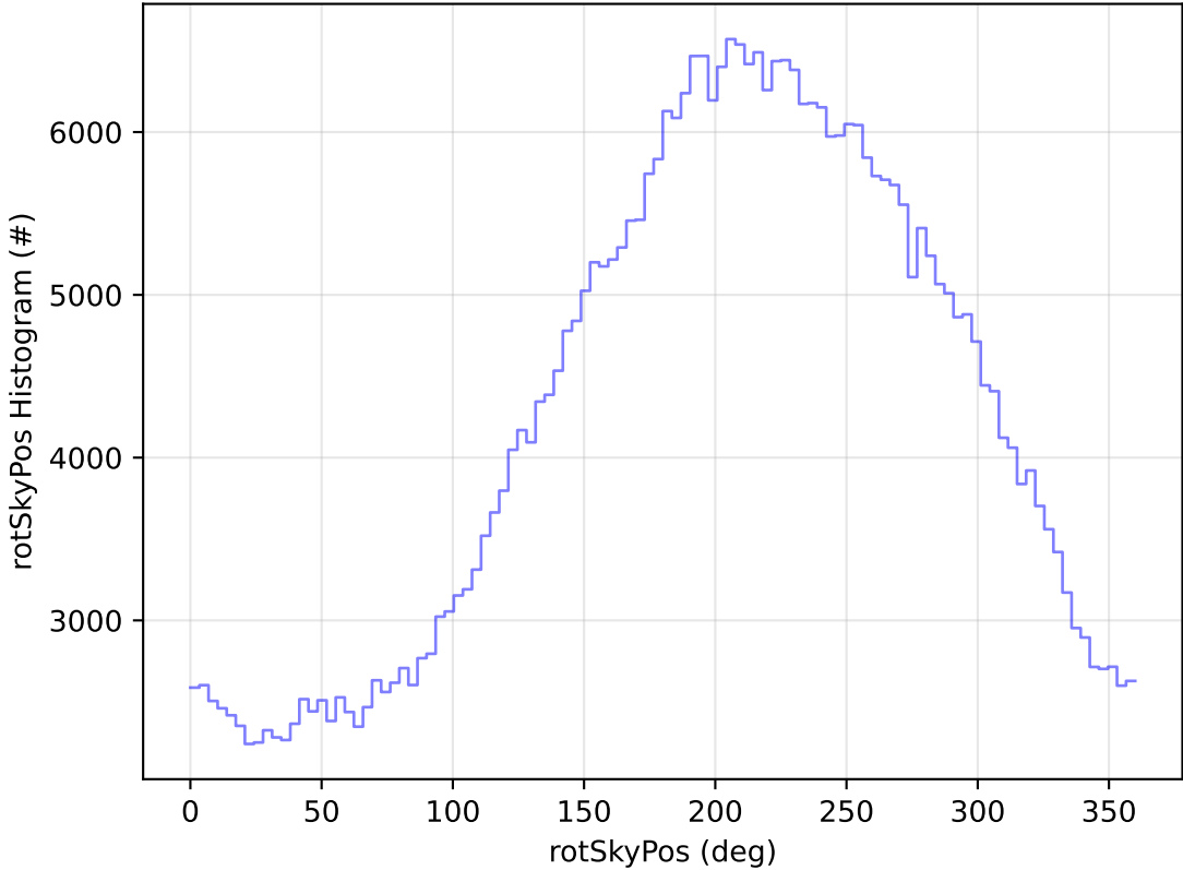
ddf_acor_sf10_lsf30_lsr10_v3.4_10yrs All sky z band: rotSkyPos Histogram
