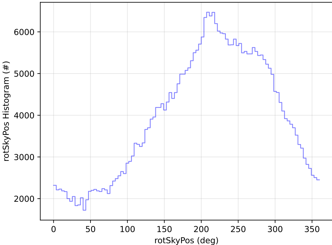
ddf_acor_sf10_lsf30_lsr10_v3.4_10yrs All sky y band: rotSkyPos Histogram
