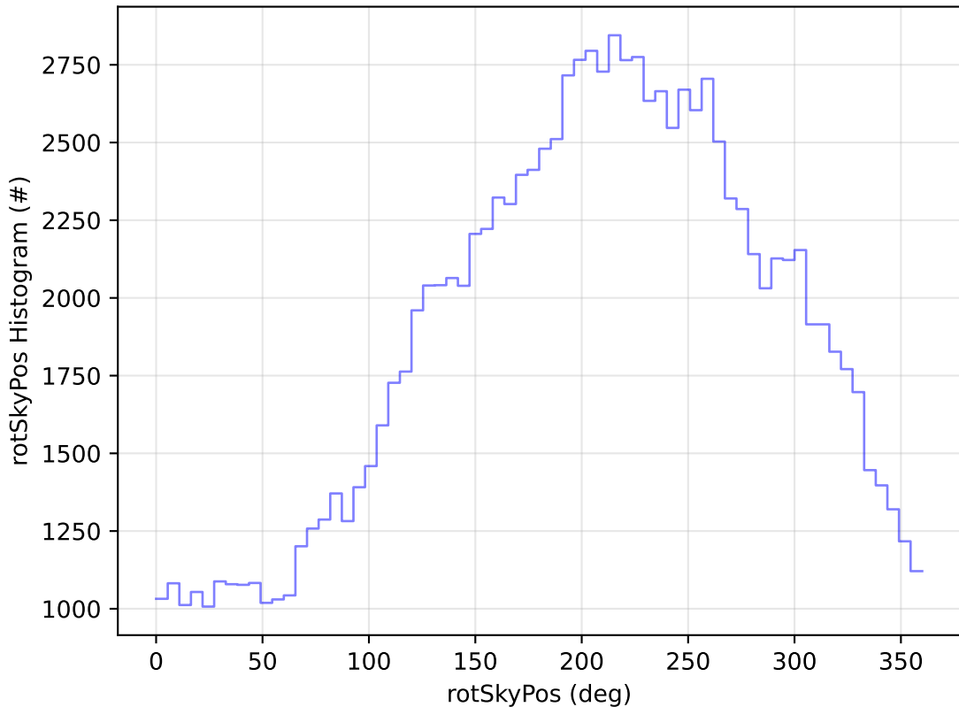
ddf_acor_sf10_lsf30_lsr10_v3.4_10yrs All sky u band: rotSkyPos Histogram
