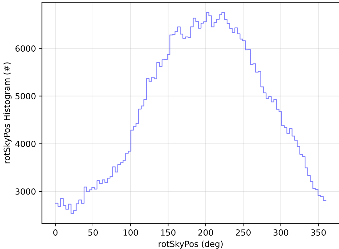
ddf_acor_sf10_ls30_lsr10_v3.4_10yrs All sky r band: rotSkyPos Histogram
