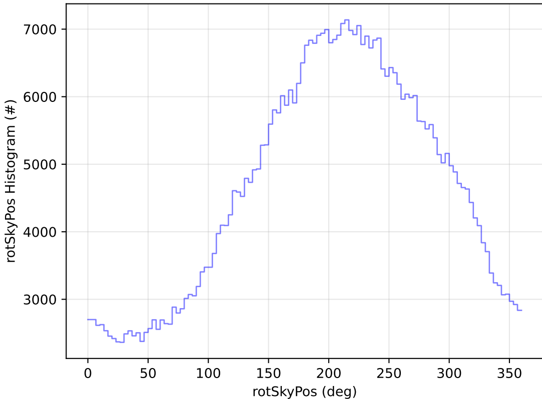
ddf_acor_sf10_lsf30_lsr10_v3.4_10yrs All sky i band: rotSkyPos Histogram
