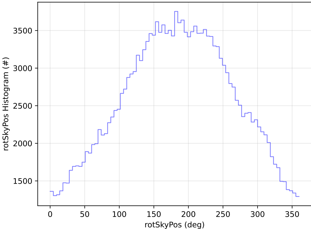
ddf_acor_sf10_lsf30_lsr10_v3.4_10yrs All sky g band: rotSkyPos Histogram
