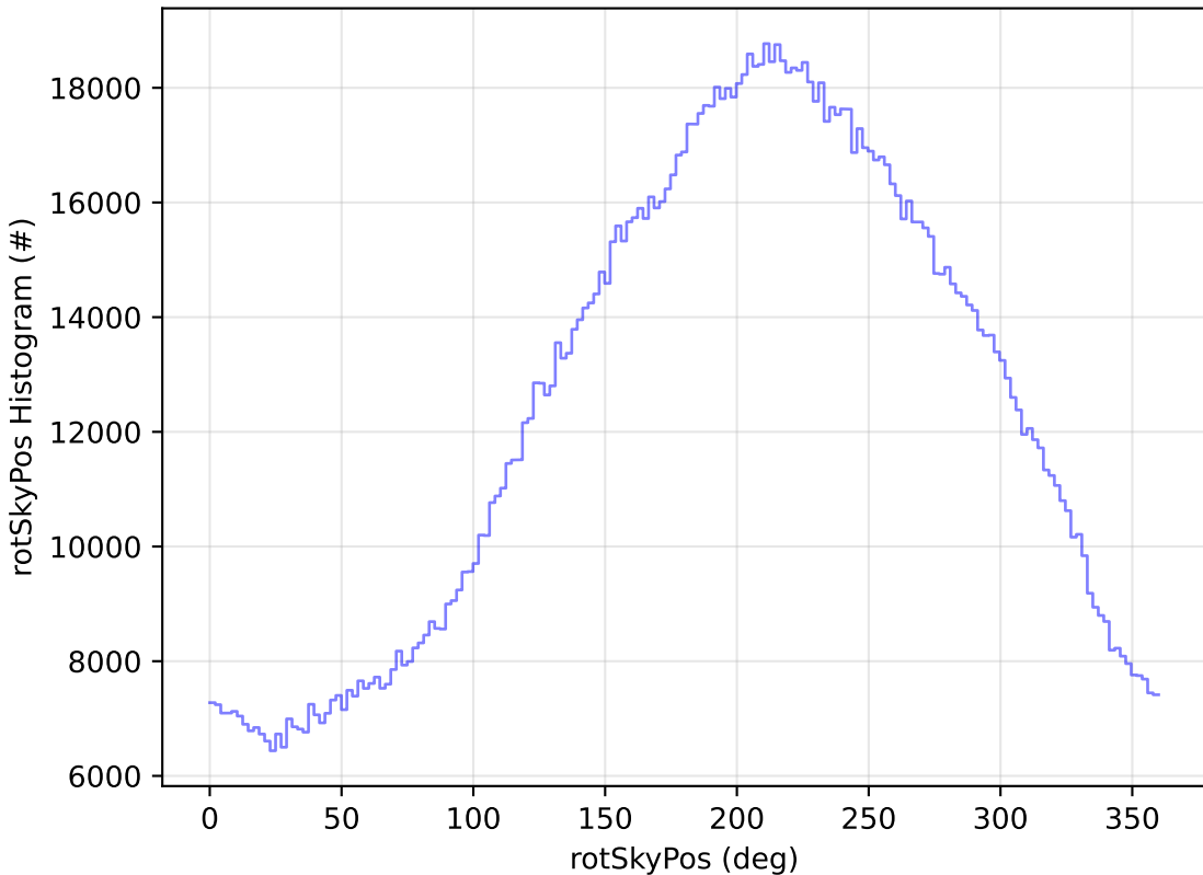
ddf_acor_sf10_lsf30_lsr10_v3.4_10yrs All sky all bands: rotSkyPos Histogram
