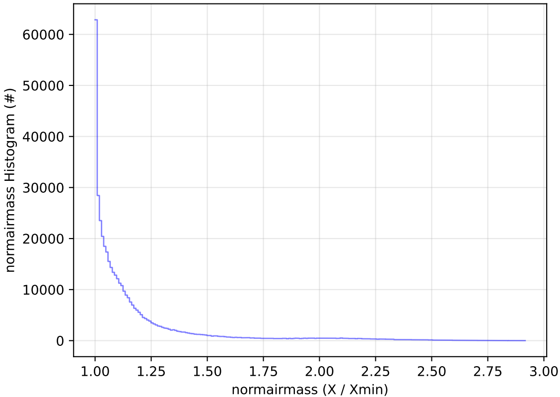
ddf_acor_sf10_lsf30_lsr10_v3.4_10yrs WFD z band: normairmass Histogram
