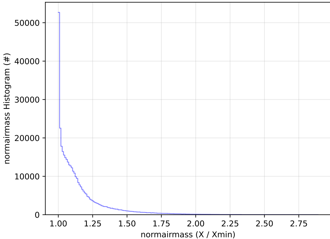
ddf_acor_sf10_lsf30_lsr10_v3.4_10yrs WFD y band: normairmass Histogram
