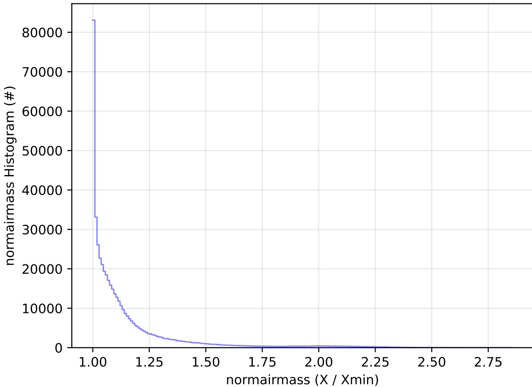
ddf_acor_sf10_lsf30_lsr10_v3.4_10yrs WFD r band: normairmass Histogram
