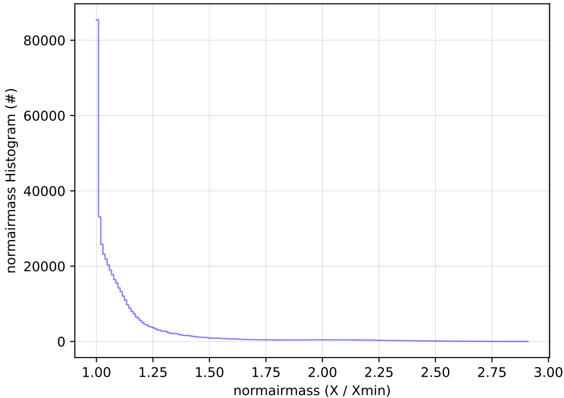
ddf_acor_sf10_lsf30_lsr10_v3.4_10yrs WFD i band: normairmass Histogram
