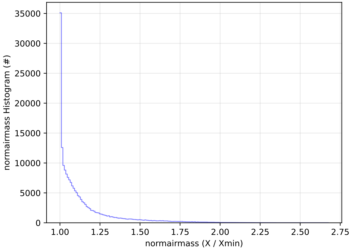
ddf_acor_sf10_lsf30_lsr10_v3.4_10yrs WFD g band: normairmass Histogram
