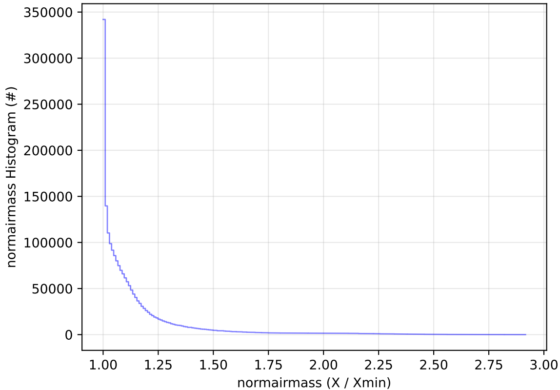
ddf_acor_sf10_lsf30_lsr10_v3.4_10yrs WFD all bands: normairmass Histogram
