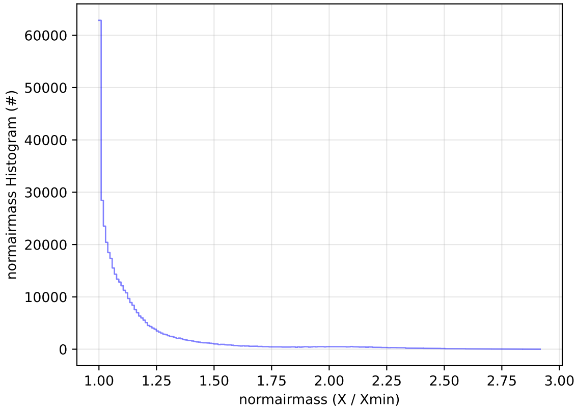
ddf_acor_sf10_lsf30_lsr10_v3.4_10yrs All sky z band: normairmass Histogram
