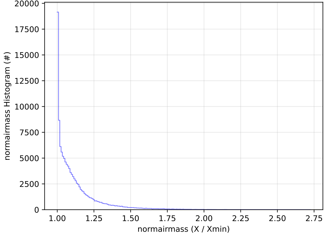
ddf_acor_sf10_lsf30_lsr10_v3.4_10yrs All sky u band: normairmass Histogram
