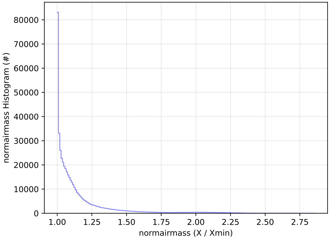
ddf_acor_sf10_lsf30_lsr10_v3.4_10yrs All sky r band: normairmass Histogram
