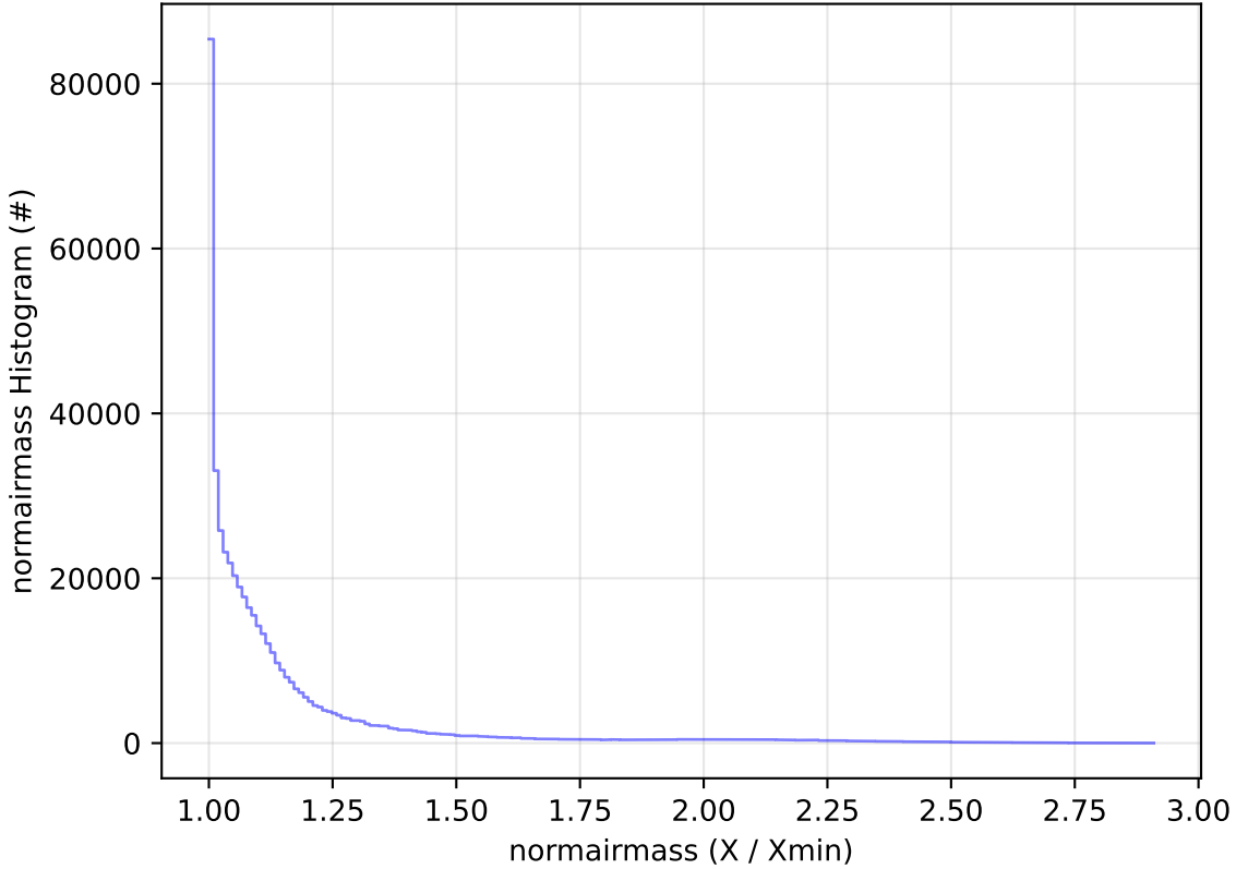
ddf_acor_sf10_lsf30_lsr10_v3.4_10yrs All sky i band: normairmass Histogram
