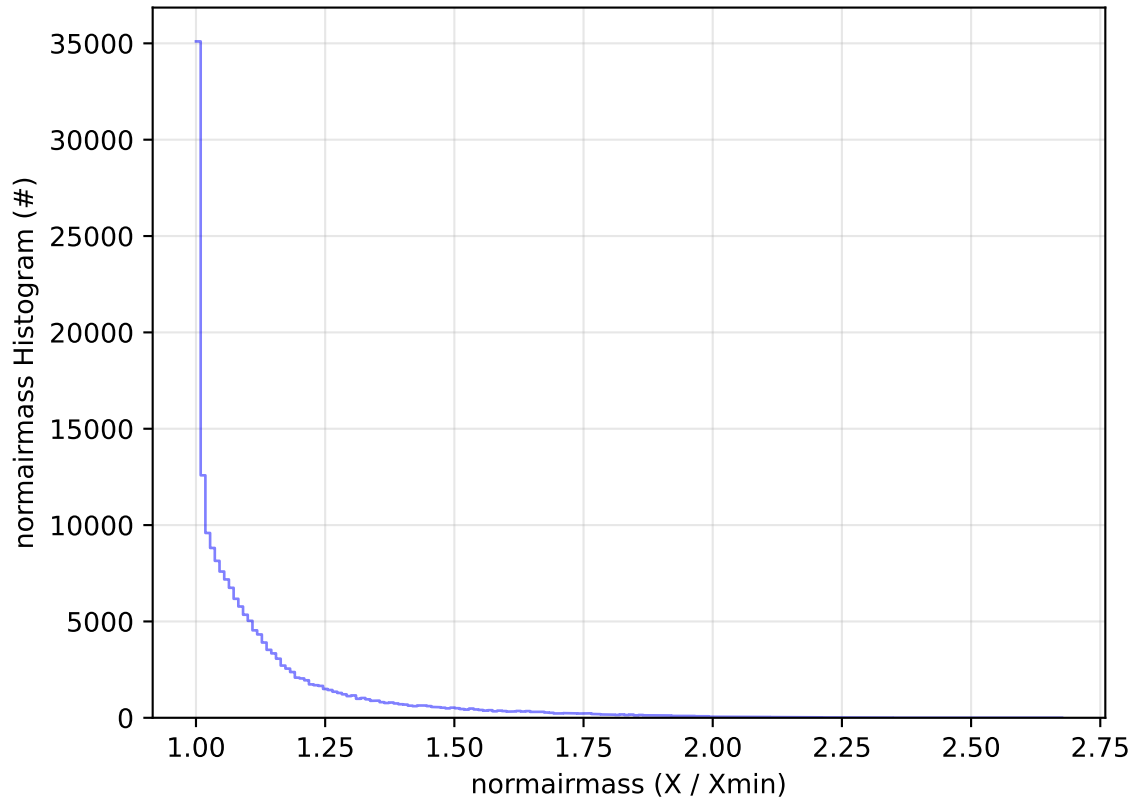
ddf_acor_sf10_lsf30_lsr10_v3.4_10yrs All sky g band: normairmass Histogram
