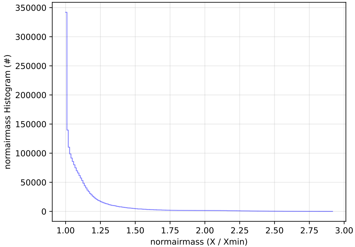
ddf_acor_sf10_lsf30_lsr10_v3.4_10yrs All sky all bands: normairmass Histogram
