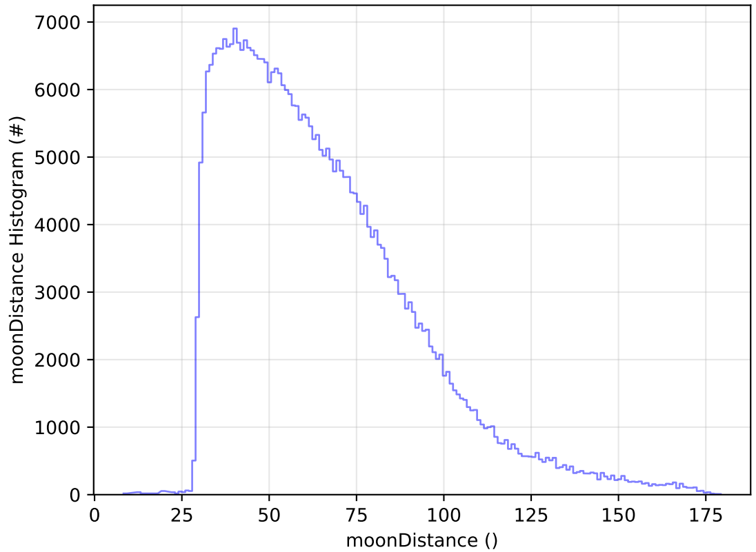
ddf_acor_sf10_lsf30_lsr10_v3.4_10yrs WFD y band: moonDistance Histogram
