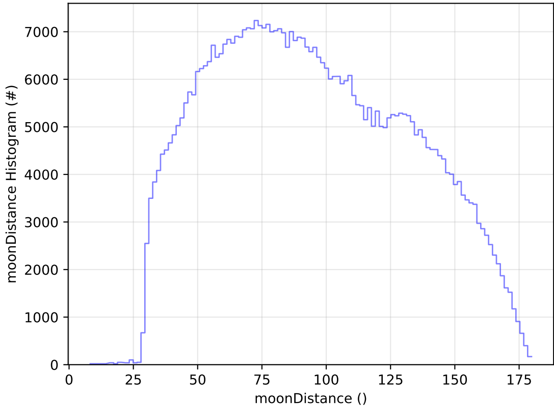
ddf_acor_sf10_lsf30_lsr10_v3.4_10yrs WFD i band: moonDistance Histogram
