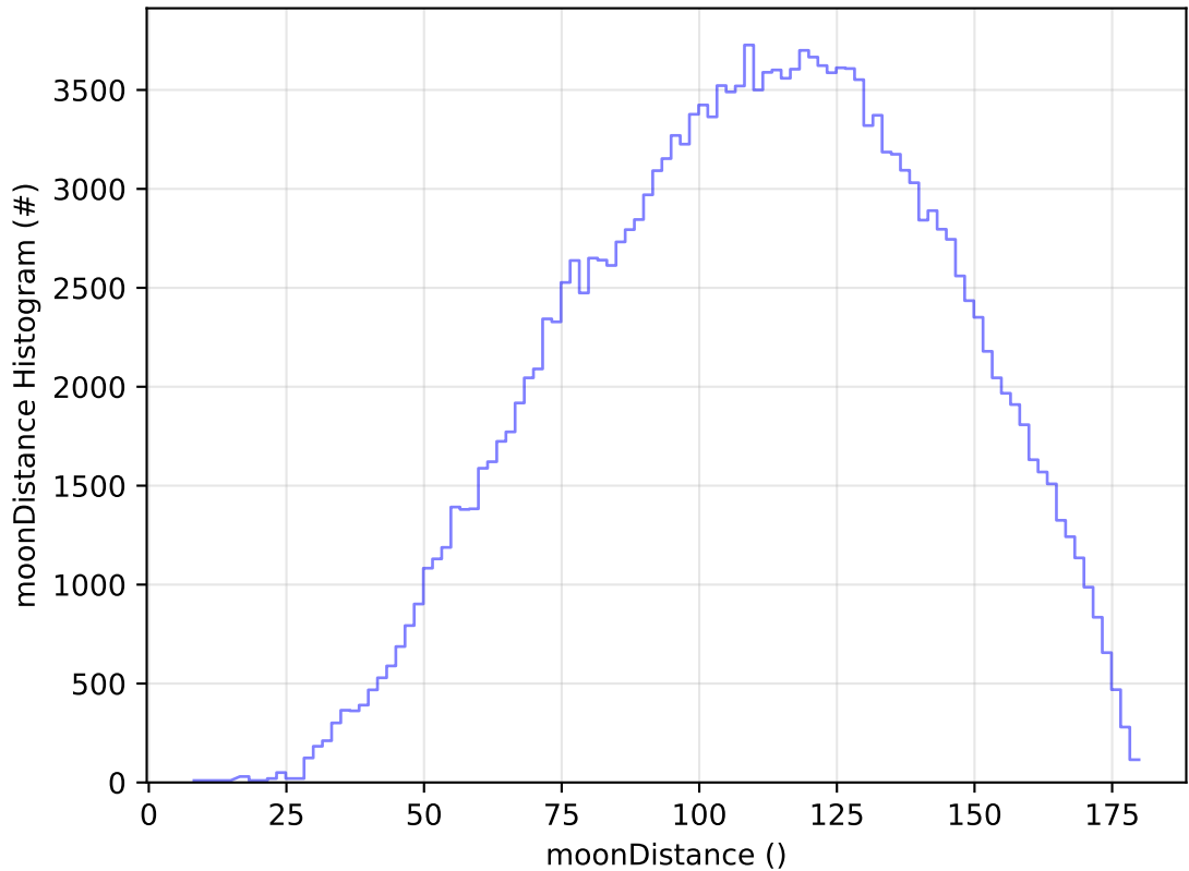
ddf_acor_sf10_lsf30_lsr10_v3.4_10yrs WFD g band: moonDistance Histogram
