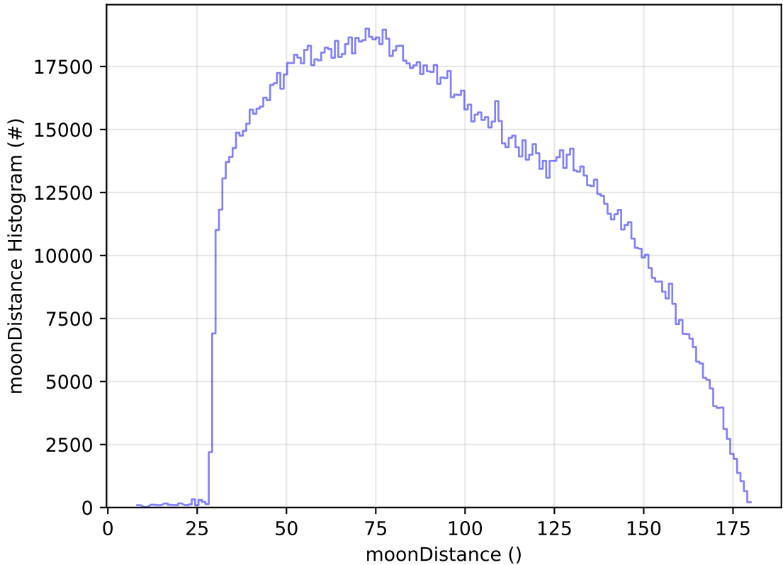
ddf_acor_sf10_lsf30_lsr10_v3.4_10yrs WFD all bands: moonDistance Histogram
