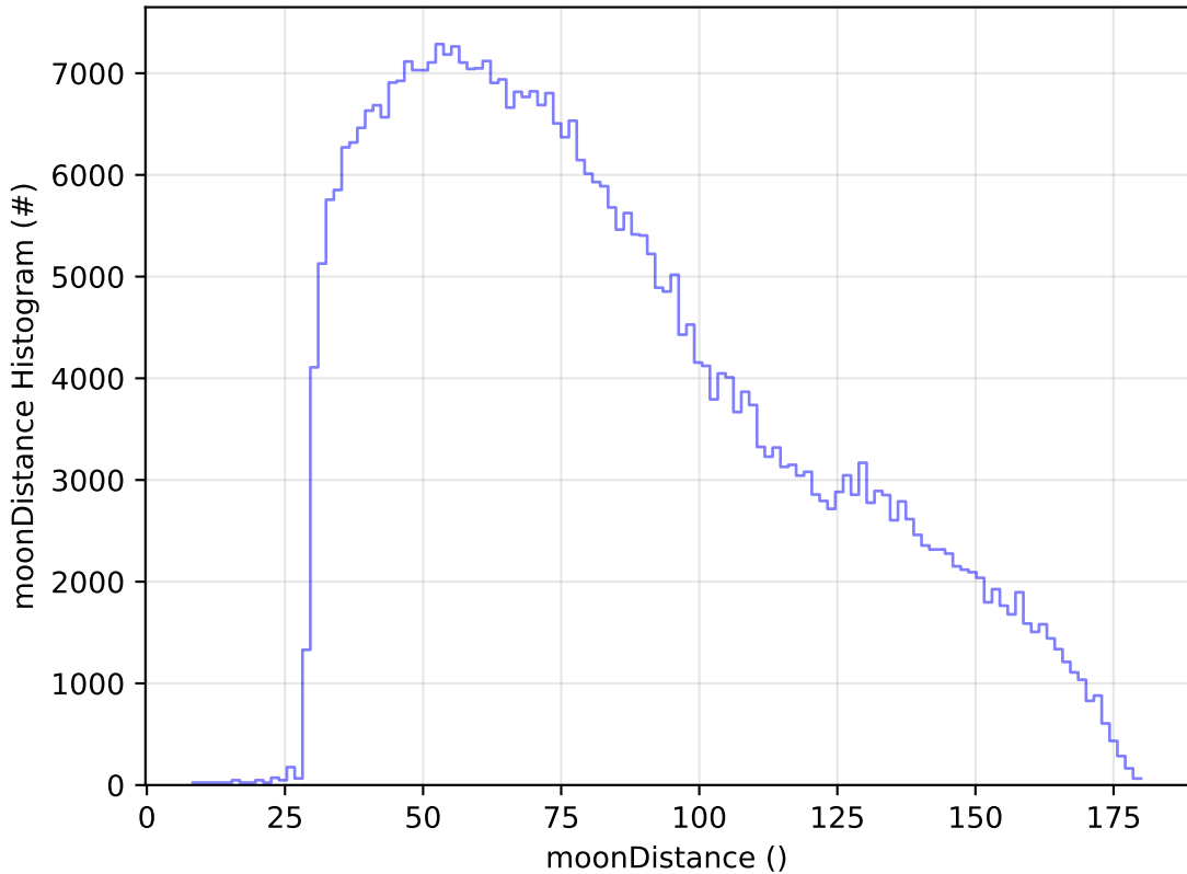
ddf_acor_sf10_lsf30_lsr10_v3.4_10yrs All sky z band: moonDistance Histogram
