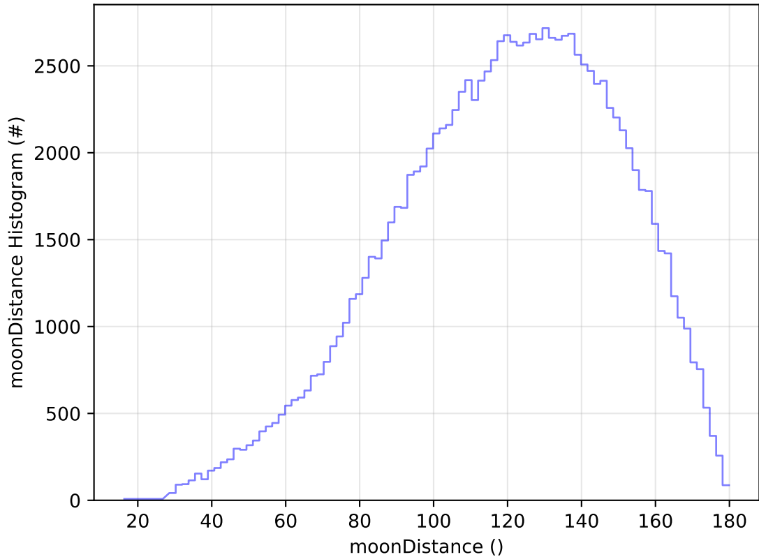
ddf_acor_sf10_lsf30_lsr10_v3.4_10yrs All sky u band: moonDistance Histogram
