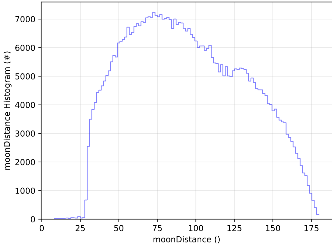
ddf_acor_sf10_lsf30_lsr10_v3.4_10yrs All sky i band: moonDistance Histogram
