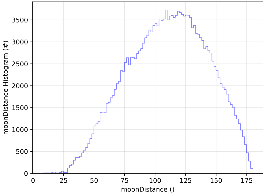
ddf_acor_sf10_lsf30_lsr10_v3.4_10yrs All sky g band: moonDistance Histogram
