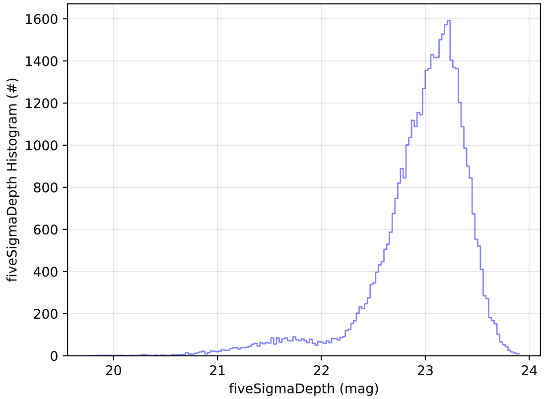
ddf_acor_sf10_lsf30_lsr10_v3.4_10yrs Yr 1 z band: fiveSigmaDepth Histogram
