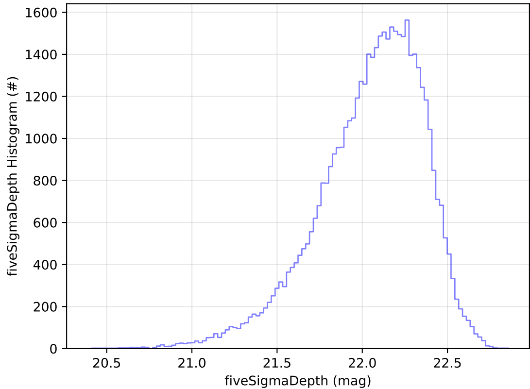
ddf_acor_sf10_lsf30_lsr10_v3.4_10yrs Yr 1 y band: fiveSigmaDepth Histogram
