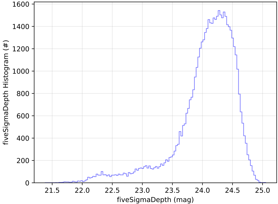
ddf_acor_sf10_lsf30_lsr10_v3.4_10yrs Yr 1 r band: fiveSigmaDepth Histogram
