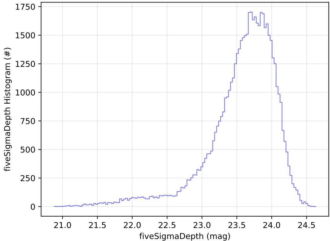
ddf_acor_sf10_lsf30_lsr10_v3.4_10yrs Yr 1 i band: fiveSigmaDepth Histogram
