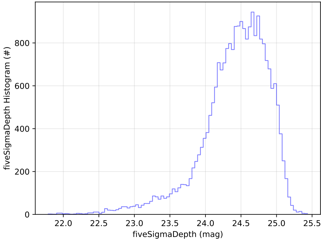
ddf_acor_sf10_lsf30_lsr10_v3.4_10yrs Yr 1 g band: fiveSigmaDepth Histogram
