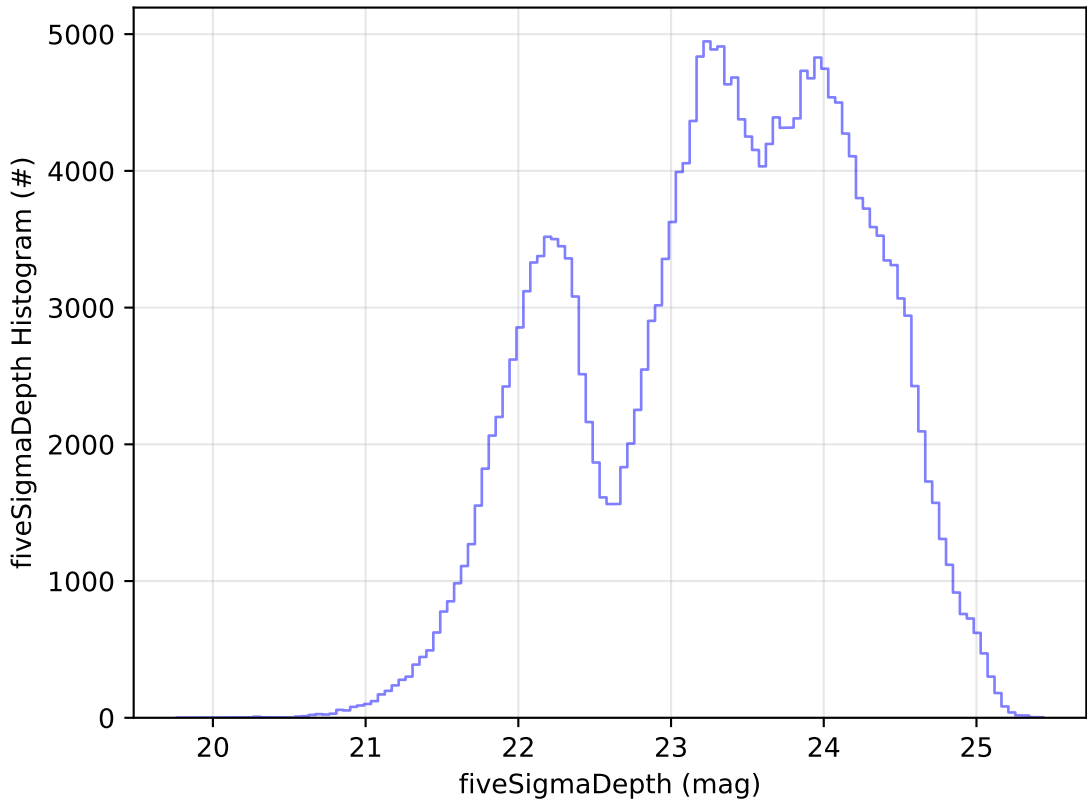
ddf_acor_sf10_Isf30_Isr10_v3.4_10yrs Yr 1 all bands: fiveSigmaDepth Histogram
