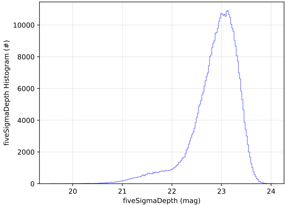
ddf_acor_sf10_lsf30_lsr10_v3.4_10yrs WFD z band: fiveSigmaDepth Histogram
