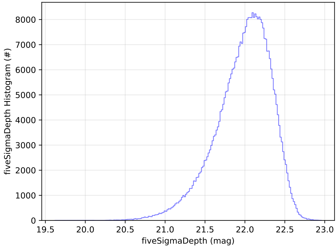
ddf_acor_sf10_lsf30_lsr10_v3.4_10yrs WFD y band: fiveSigmaDepth Histogram
