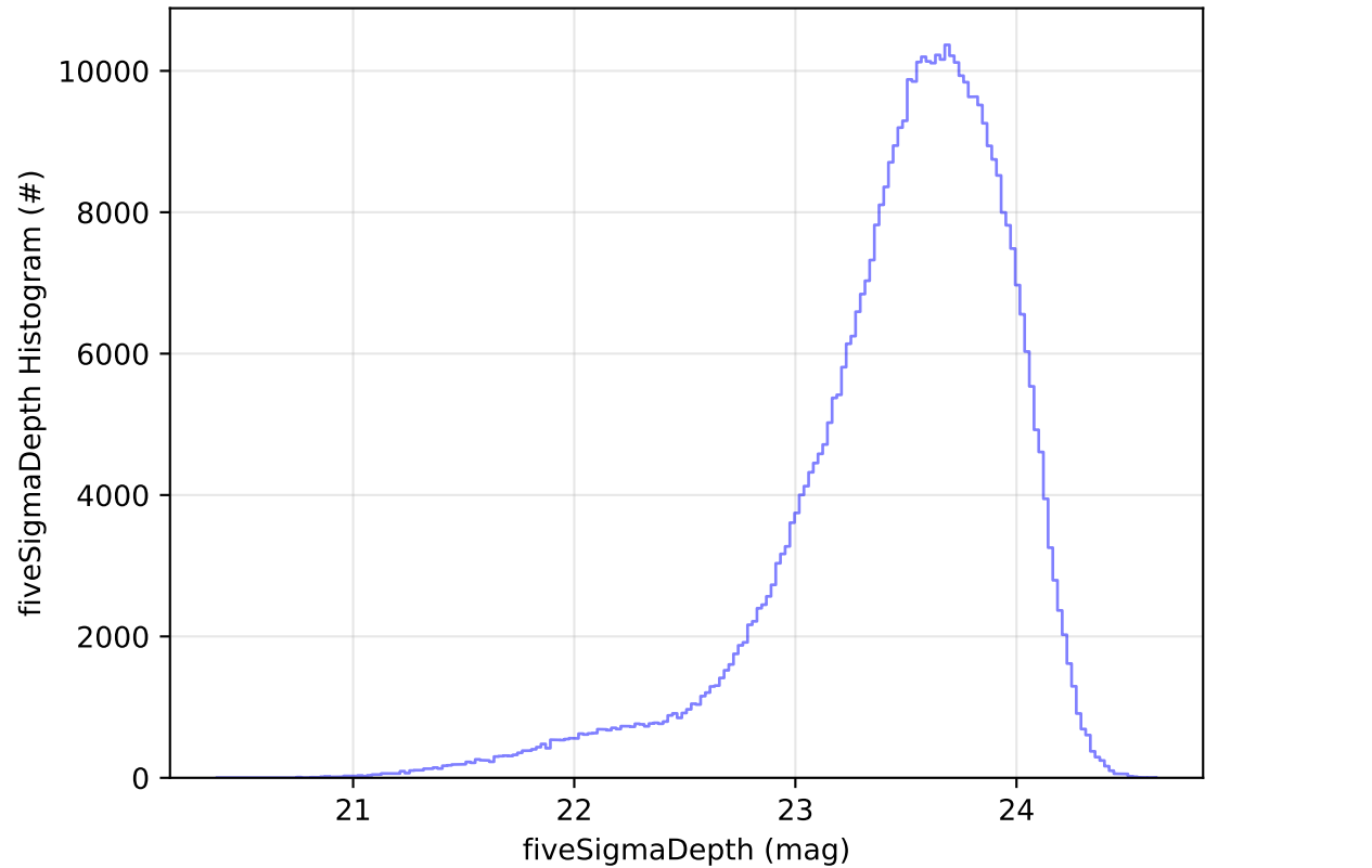
ddf_acor_sf10_lsf30_lsr10_v3.4_10yrs WFD i band: fiveSigmaDepth Histogram
