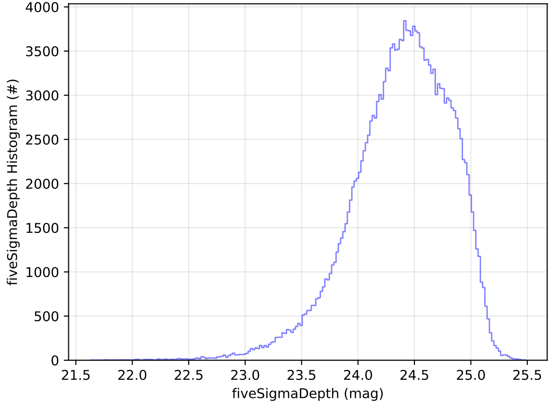
ddf_acor_sf10_lsf30_lsr10_v3.4_10yrs WFD g band: fiveSigmaDepth Histogram
