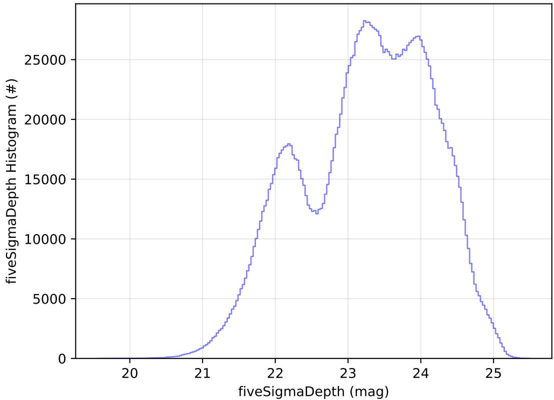
ddf_acor_sf10_lsf30_lsr10_v3.4_10yrs WFD all bands: fiveSigmaDepth Histogram
