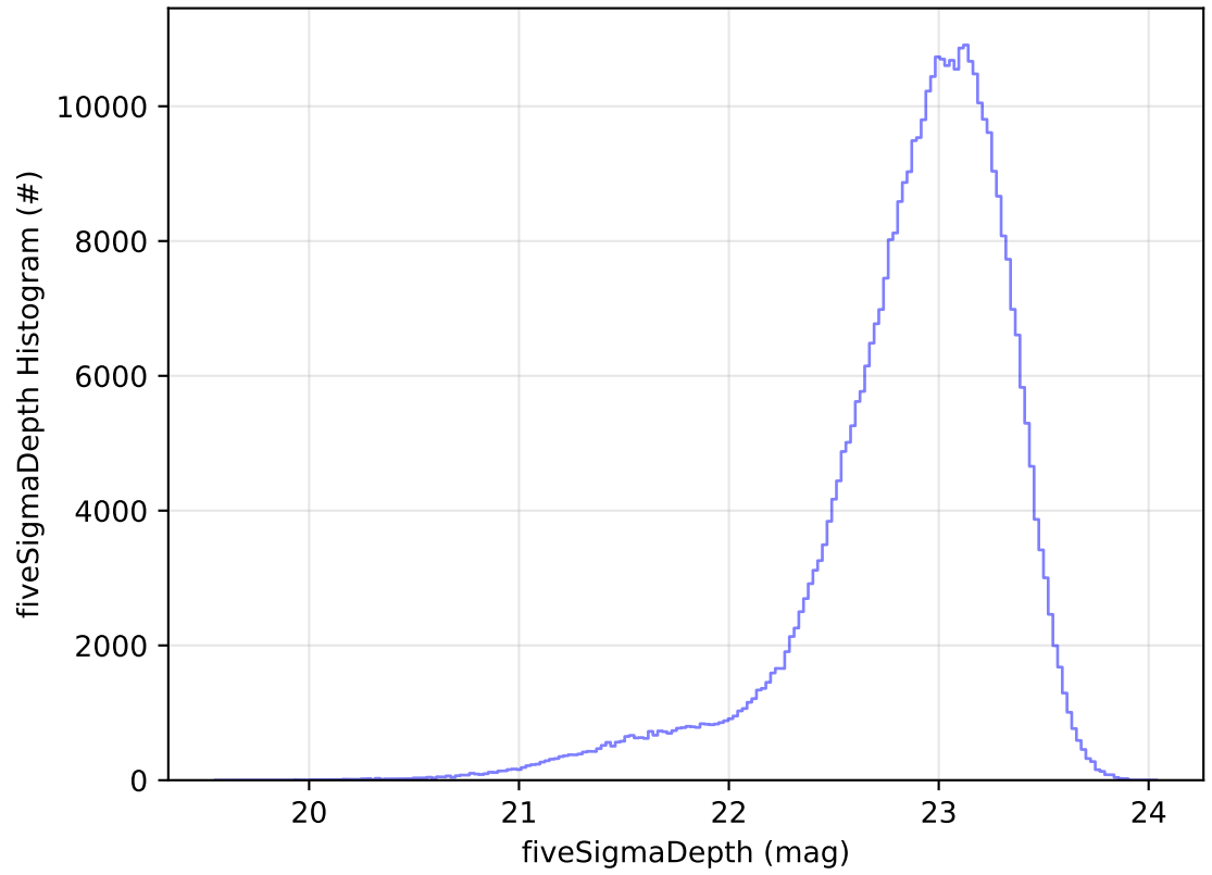
ddf_acor_sf10_lsf30_lsr10_v3.4_10yrs All sky z band: fiveSigmaDepth Histogram
